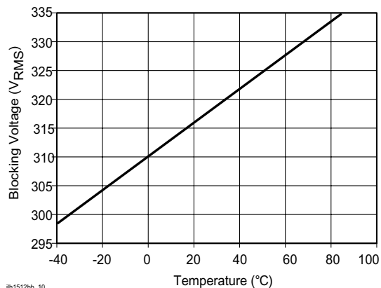
Figure 10. Form B_Typical Blocking Voltage vs. Temperature
