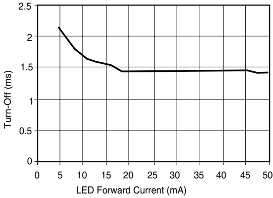
Figure 17. Form B_Typical Turn-Off vs. LED Forward Current
