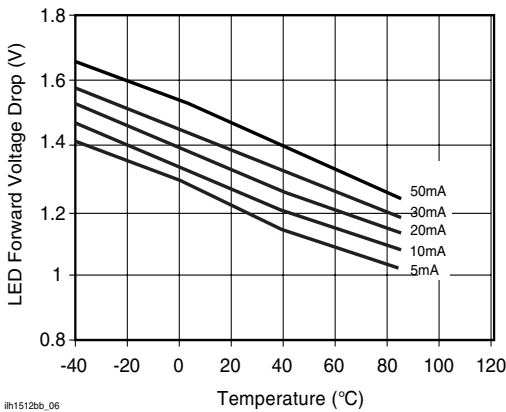
Figure 6. Typical LED Forward Voltage Drop vs. Temperature
