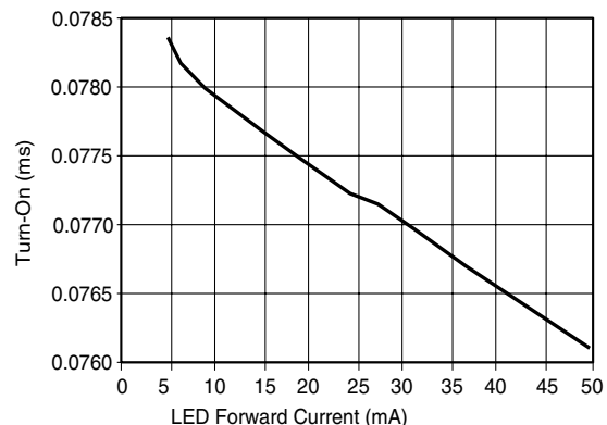
Figure 16. Form B_Typical Turn-On vs. LED Forward Current
