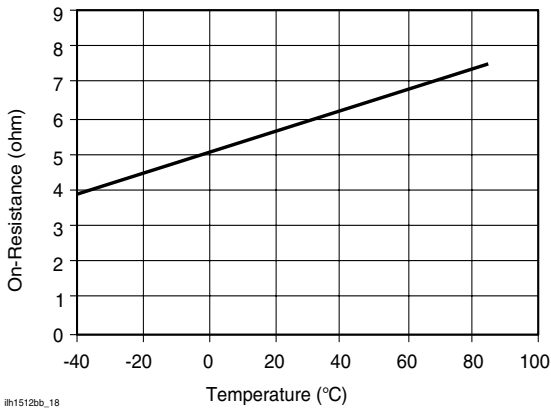
Figure 18. Form B_Typical On-Resistance vs. Temperature
