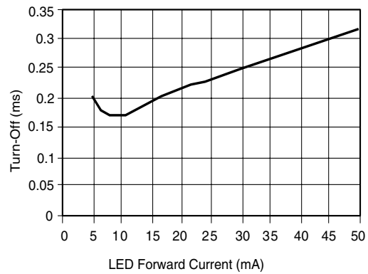
Figure 14. Form A_Typical Turn-Off vs. LED Forward Current
