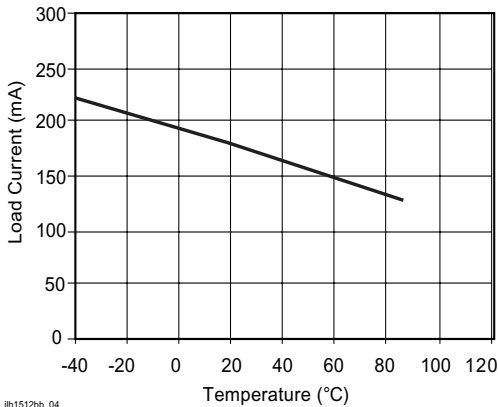
Figure 5. Form B_Typical Load Current vs. Temperature
