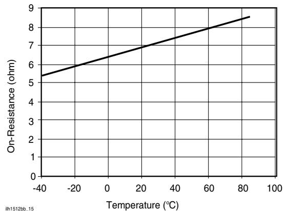
Figure 15. Form A_Typical On-Resistance vs. Temperature
