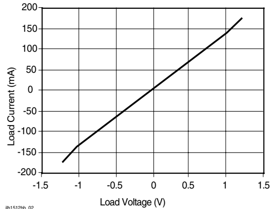
Figure 3. Form A_Typical Load Current vs. Load Voltage
