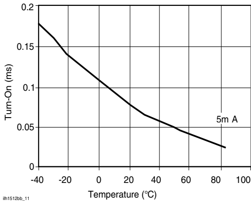
Figure 11. Form B_Typical Turn-On vs. Temperature
