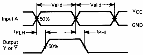
Figure 3. Switching Waveforms
