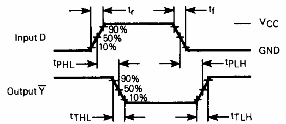
Figure 2. Switching Waveforms
