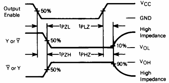
Figure 4. Switching Waveforms
