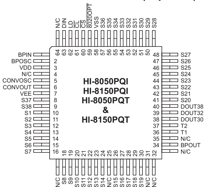
64 Pin plastic PQFP
