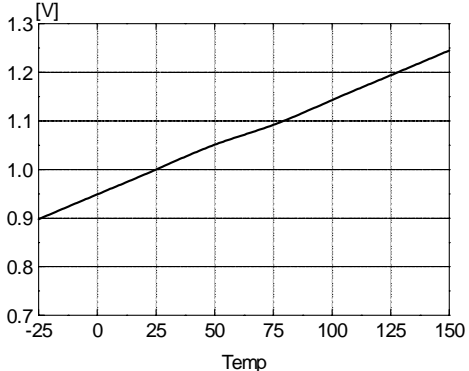
Figure 16. Burst Mode Enable Voltage vs. Temp.
