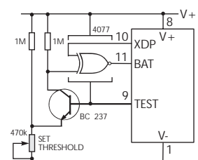
Check Link BAT is OPEN.
