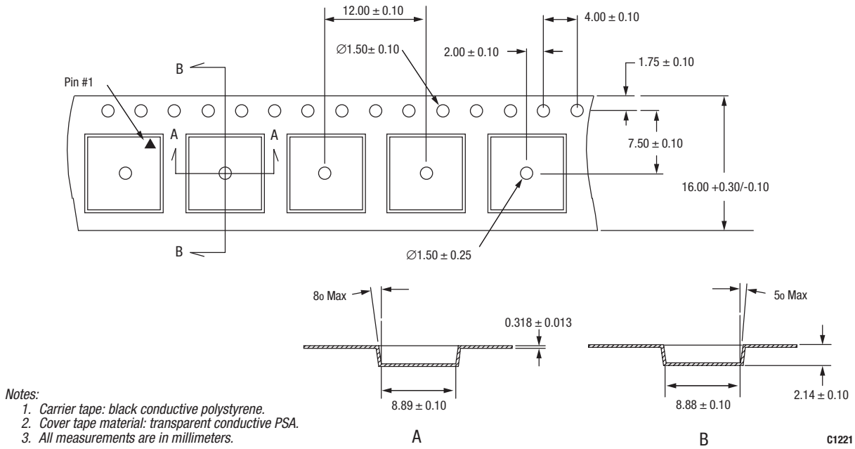
Figure 10. CX65105 8-Pin LCC Tape and Reel Dimensions
