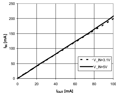
Figure 9. I_{IN} vs. I_{OUT}
