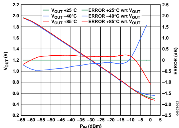
Figure 34. Error vs. Temperature with Respect to Output Voltage at 25°C (Does Not Take Transfer Function Nonlinearities at 25°C into Account)
