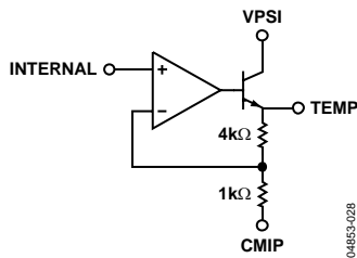
Figure 29. Temp Sensor Interface
