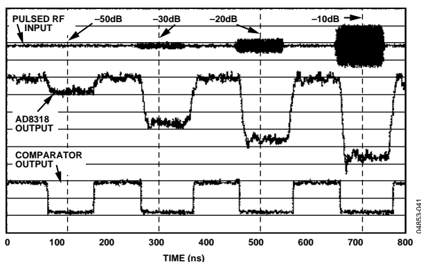
Figure 39. Pulse Response of AD8318 and Comparator for RF Pulses of Varying Amplitudes
