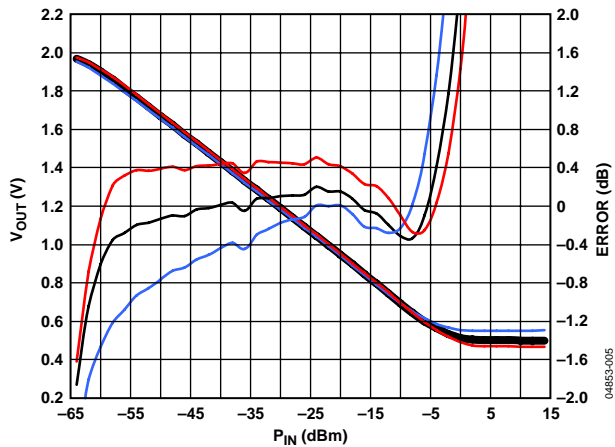
Figure 5. V_{OUT} and Log Conformance vs. Input Amplitude at 2.2 GHz, Typical Device
