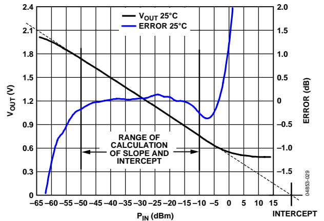
Figure 30. Typical Output Voltage vs. Input Signal
