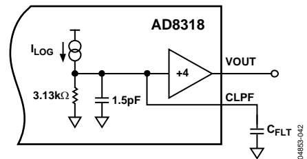
Figure 40. Lowering the Postdemodulation Bandwidth
