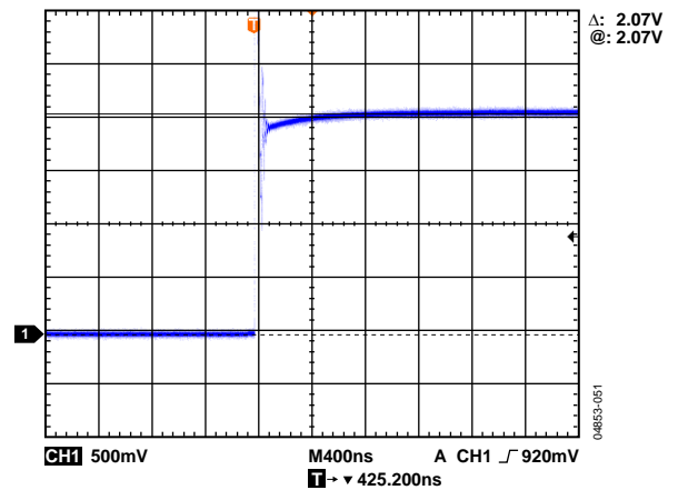
Figure 24. ENBL Response Time; V POS = 5.0 V; Input AC-Coupling Caps = 18 pF; C LPF = Open
