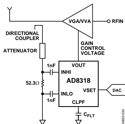
Figure 41. AD8318 Controller Mode
