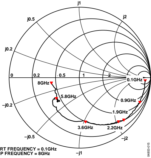
Figure 15. Input Impedance vs. Frequency; No Termination Resistor on INHI, Z_0 = 50\ \Omega
