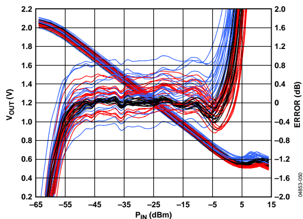
Figure 35. Output Voltage and Error vs. Temperature (+25°C, -40°C, and +85°C) of a Population of Devices Measured at 5.8 GHz
