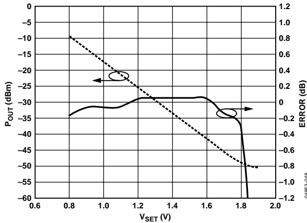
Figure 43. AD8367 Output Power vs. AD8318 Setpoint Voltage
