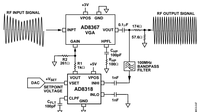
Figure 42. AD8318 Operating in Controller Mode to Provide Automatic Gain Control Functionality in Combination with the AD8367
