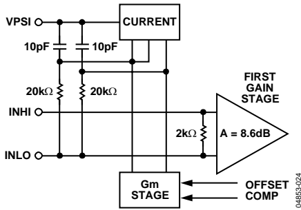
Figure 25. Input Interface
