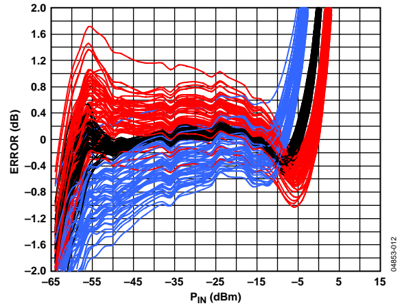
Figure 12. Distribution of Error at Temperature After Ambient Normalization vs. Input Amplitude at 3.6 GHz for at Least 70 Devices, R_{TADJ} = 51 \Omega
