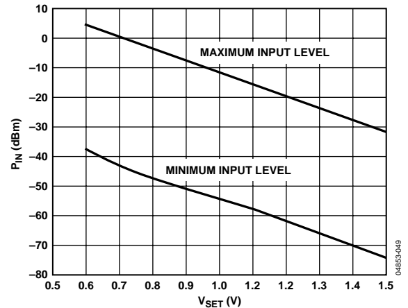
Figure 45. Setpoint Voltage vs. Input Power. Optimal signal levels must be used to achieve the full 45 dB dynamic range capabilities of the AD8367.
