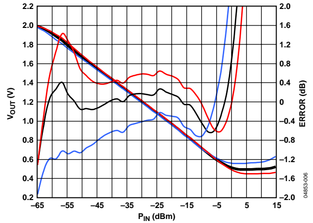
Figure 6. V_{OUT} and Log Conformance vs. Input Amplitude at 3.6 GHz, Typical Device, R_{TADJ} = 51\ \Omega
