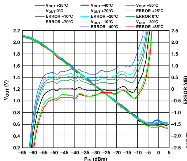
Figure 36. Typical Drift at 5.8 GHz for Various Temperatures
