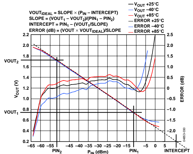
Figure 31. Transfer Function at 2.2 GHz
