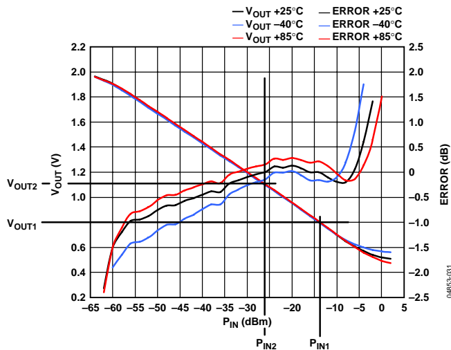
Figure 32. Output Voltage and Error vs. P_{\text{IN}} with 2-Point Calibration at -10 dBm and -30 dBm
