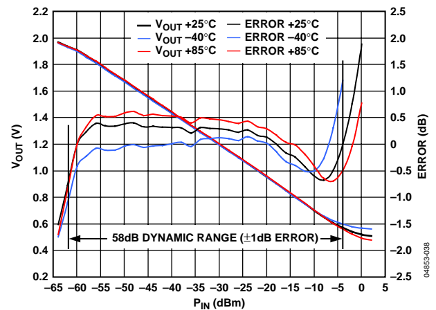
Figure 33. Dynamic Range Extension by Choosing Calibration Points Close to the End of the Linear Range
