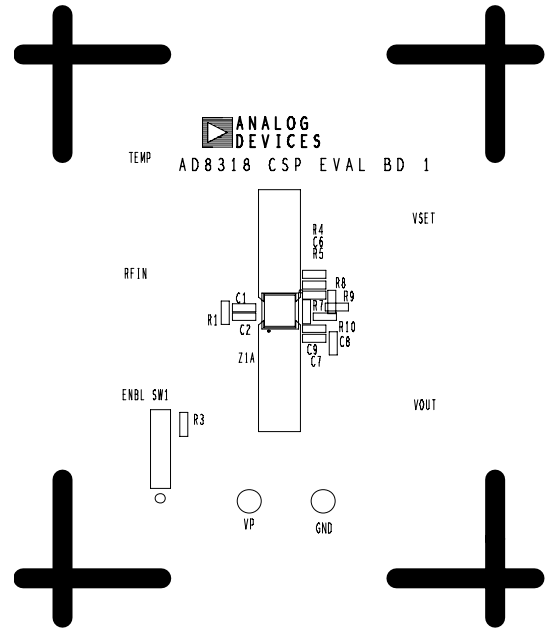
Figure 49. Component Side Silkscreen
