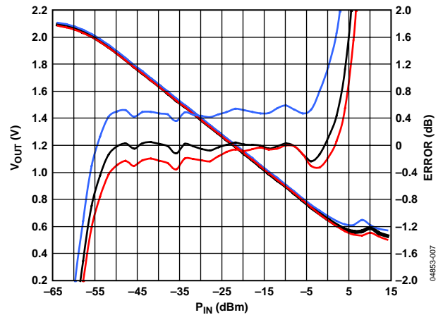
Figure 7. V_{OUT} and Log Conformance vs. Input Amplitude at 5.8 GHz, Typical Device, R_{TADJ} = 1000\ \Omega
