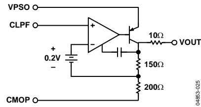
Figure 26. Output Interface
