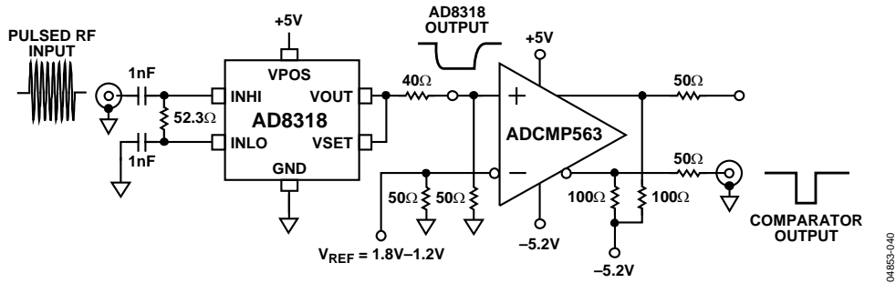
Figure 38. AD8318 Operating with the High Speed ADCMP563 Comparator
