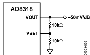
Figure 37. Increasing the Slope
