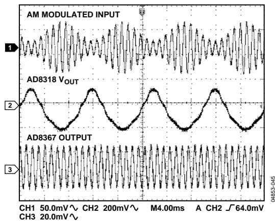
Figure 44. Oscilloscope Screen Image Showing an AM Modulated Input Signal to the AD8367. The AD8318 tracks the envelope of this input signal and applies the appropriate voltage to ensure a constant output from the AD8367.
