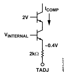
Figure 28. TADJ Interface
