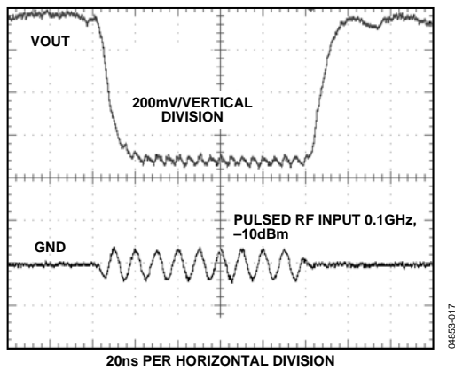
Figure 17. V_{OUT} Pulse Response Time; Pulsed RF Input 0.1 GHz, -10 dBm; C_{LPF} = \text{Open}
