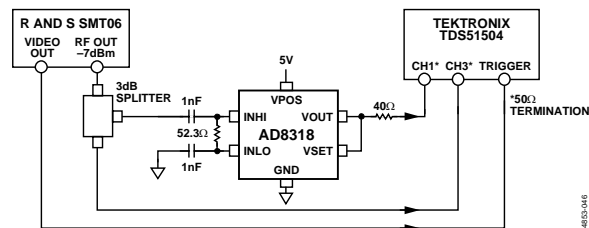
Figure 46. Pulse Response Measurement Test Setup
