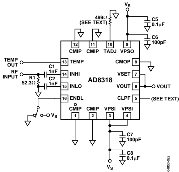
Figure 22. Basic Connections
