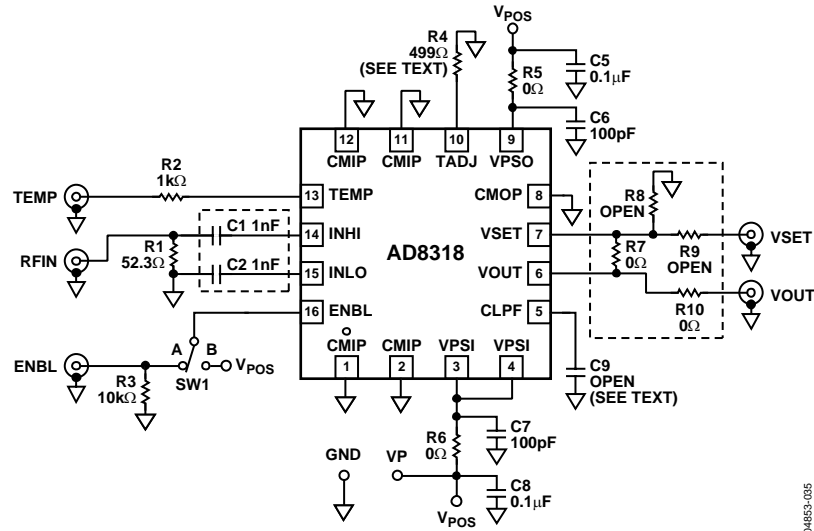
Figure 47. Evaluation Board Schematic
