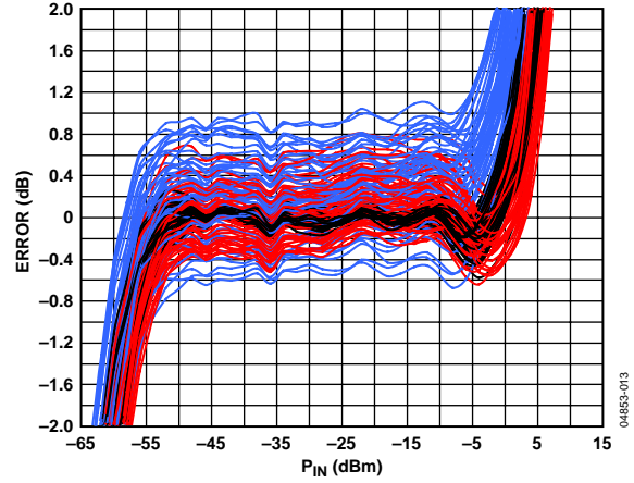
Figure 13. Distribution of Error at Temperature After Ambient Normalization vs. Input Amplitude at 5.8 GHz for at Least 70 Devices, R_{TADJ} = 1000 \Omega
