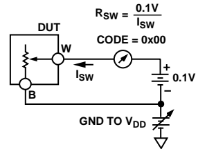
Figure 36. Test Circuit for Common-Mode Leakage Current
