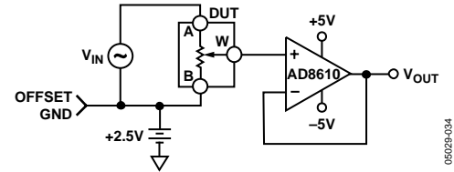
Figure 35. Test Circuit for Gain vs. Frequency
