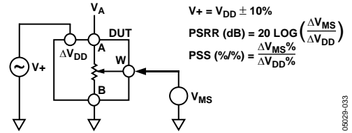
Figure 34. Test Circuit for Power Supply Sensitivity (PSS, PSSR)
