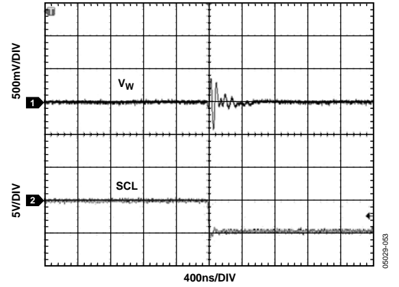
Figure 28. Digital Feedthrough
