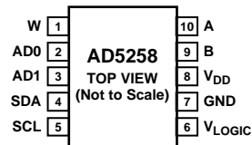
Figure 3. Pinout
