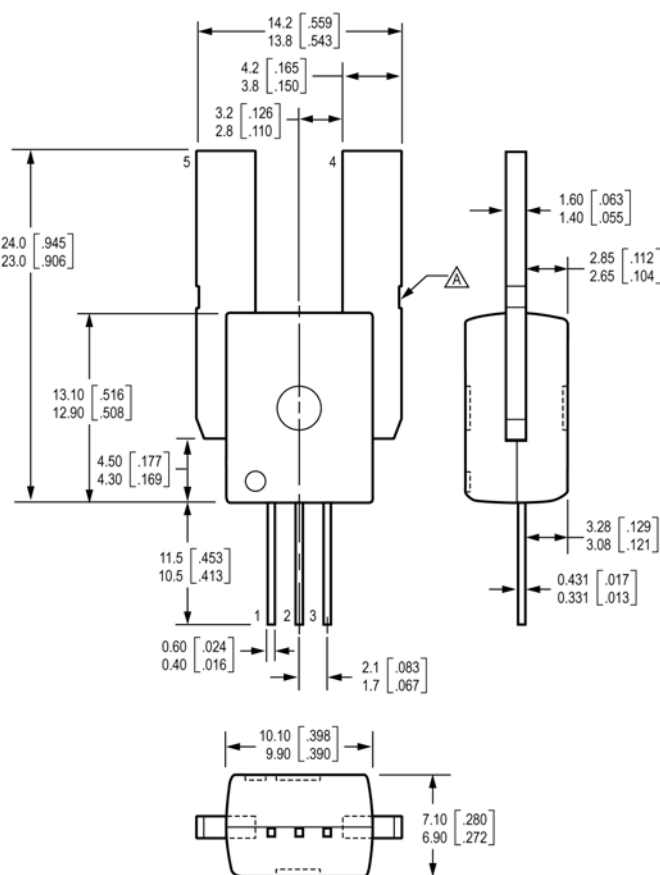
Package CB-PSS
