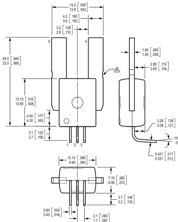
Package CB-PSF
