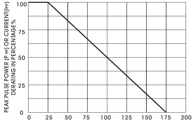
FIGURE 2 DERATING CURVE
