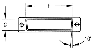
Rear Shell (Plug & Receptacle)
