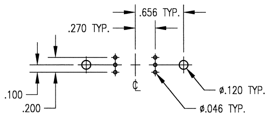
2W2 Straight Coax Contacts
