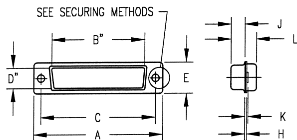
Plug Shell
