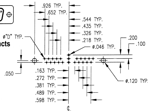
13W6 Right Angle Coax Contacts
