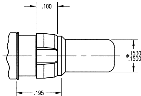
Plug Interface
