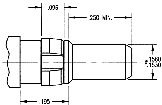
Plug Interface
