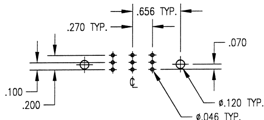
3W3 Right Angle Coax Contacts
