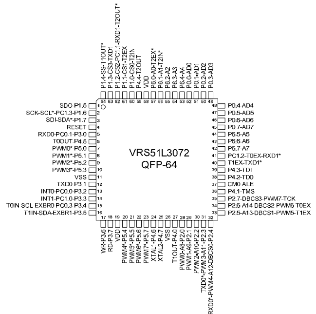
FIGURE 2: VRS51L3072 QFP-64
