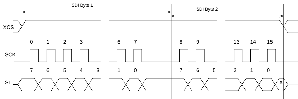
Figure 9: Two SDI Bytes.
