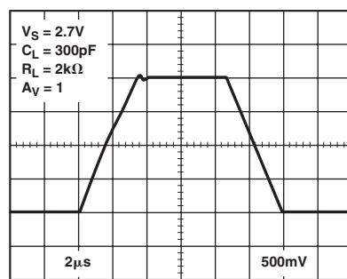
TPC 17. Large Signal Transient Response at 2.7 V
