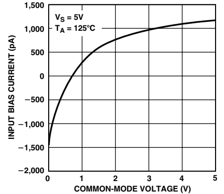
TPC 3. Input Bias Current vs. Common-Mode Voltage
