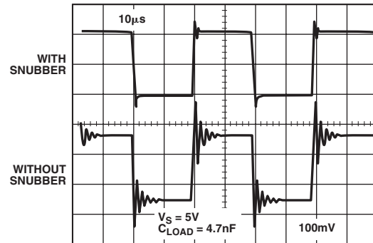
Figure 10. Overshoot and Ringing are Substantially Reduced Using a Snubber Network
