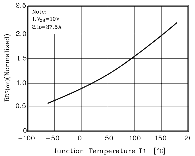
Fig.8 R_{DS(on)} - T_J
