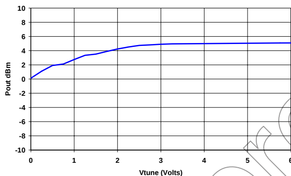
XQ1001-BD Output Power vs. Tuning Voltage
