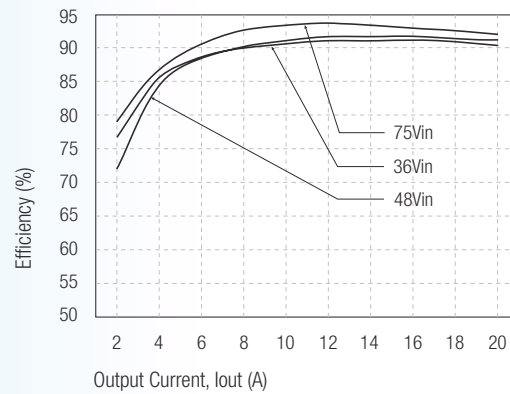
Input With Heatsink (7G-0022) RP100-4805SB
