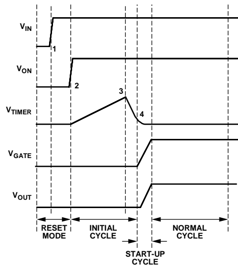
Figure 36. Power-Up Timing
