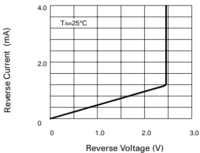
Reverse Characteristics
