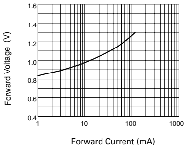
Forward Characteristics
