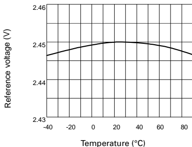
Temperature Drift
