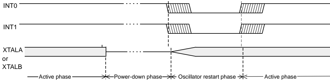
Figure 31. Power-down Exit Waveform
