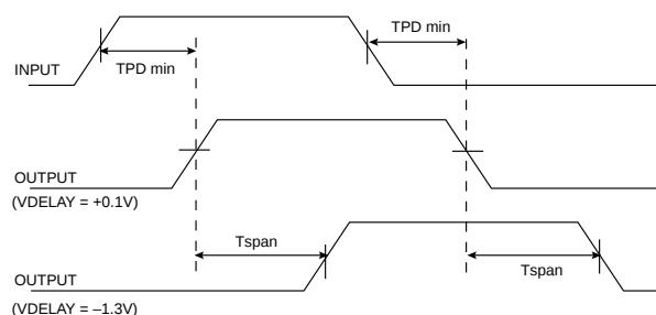
Figure 2. VDELAY Control
