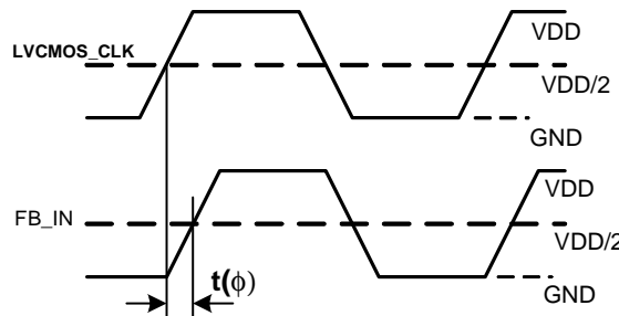
Figure 4. LVC MOS Propagation Delay t(φ), Static Phase Offset
