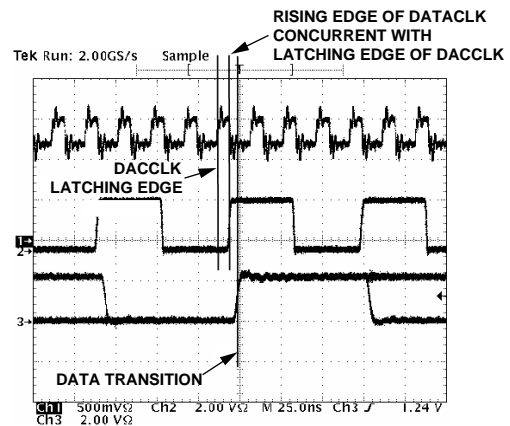
Figure 43. DATAADJ = 1111
