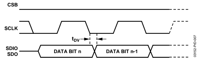
Figure 33. Timing Diagram for Register Read
