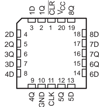
SN54LV273A . . . FK PACKAGE (TOP VIEW)
