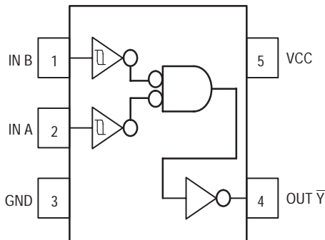
Figure 1. 5-Lead SOT-353 Pinout (Top View)
