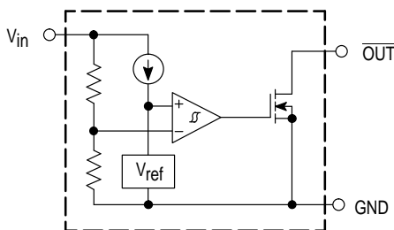
MC33460 Nch Open Drain Configuration
