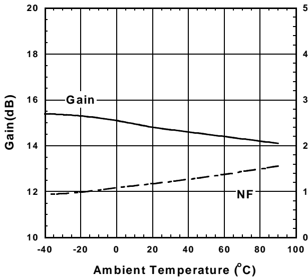
Gain, Noise Figure vs. Temperature
