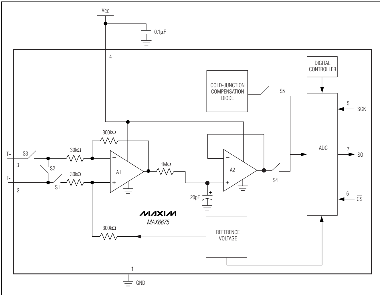
Block Diagram
