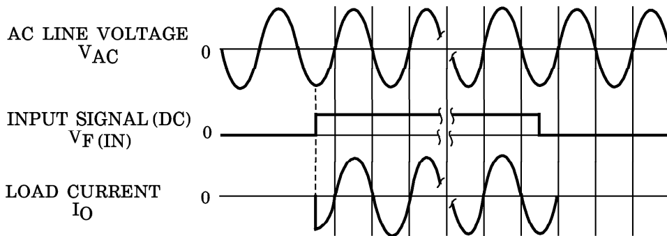
Fig.1 SWITCHING WAVEFORM
