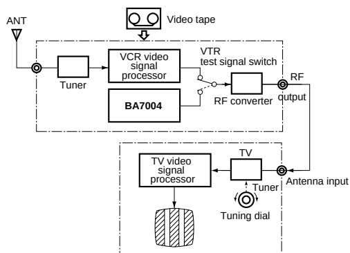
Fig. 3 Connection example
