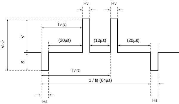
Fig. 2 Output waveform
