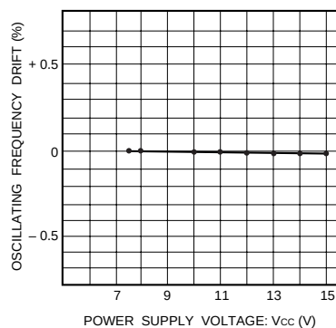
Fig. 4 Oscillation frequency vs. power supply voltage
