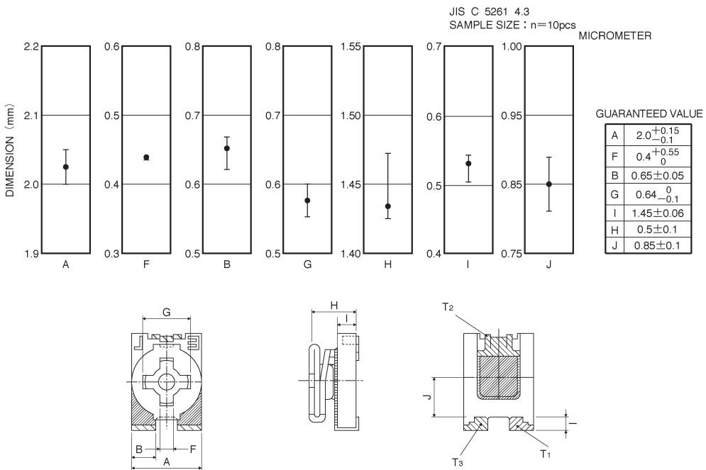
Fig.2 Dimensions
