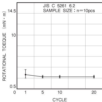
Fig. 7 Rotational torque
