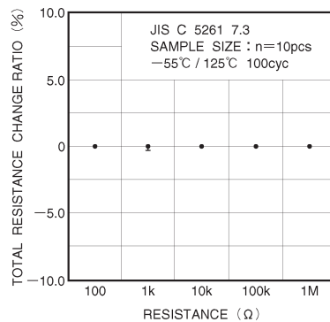
Fig.10-1 Temperature cycling
