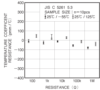
Fig.5 Resistance temperature characteristics
