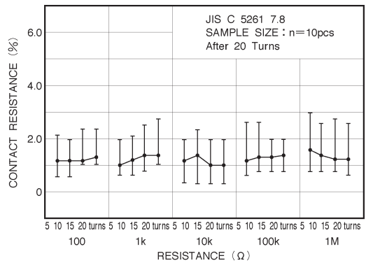
Fig.6-2 Endurance (wiper)
