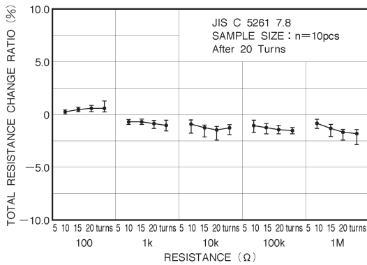
Fig.6-1 Endurance (wiper)
