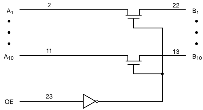
Figure 2. Logic Diagram
