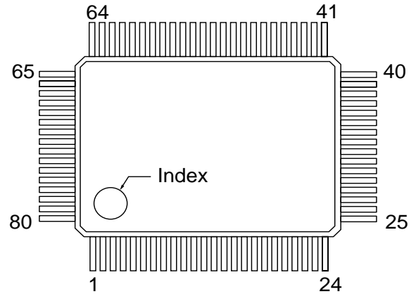
top view 80-pin Gullwing Package
