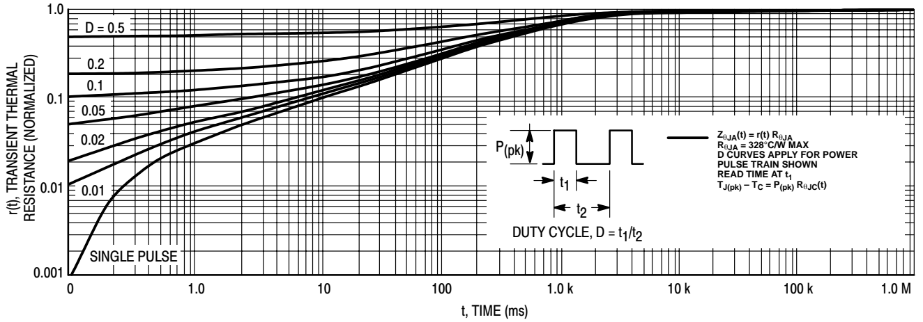
Figure 25. Thermal Response
