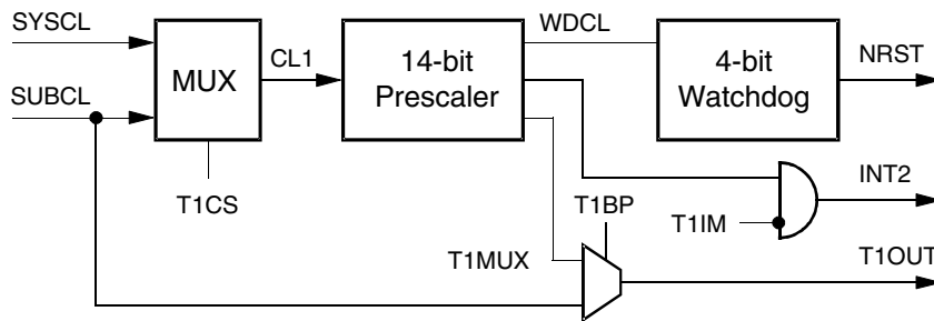
Figure 5-7. Timer 1 Module
