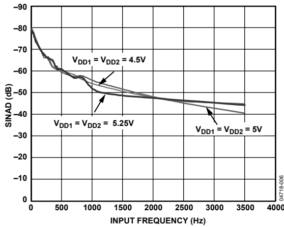
Figure 7. SINAD vs. Analog Input Frequency for Various Supply Voltages
