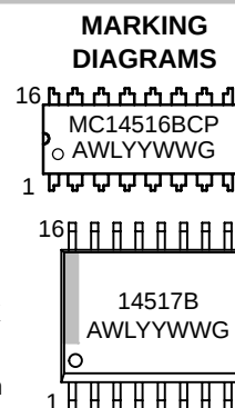
SOIC-16 DW SUFFIX CASE 751G
