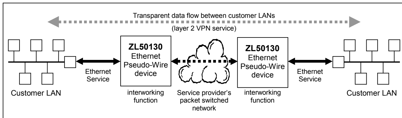
Figure 3 - ZL50130 Operation
