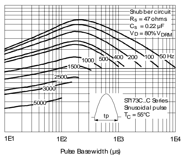
Fig. 13 - Frequency Characteristics
