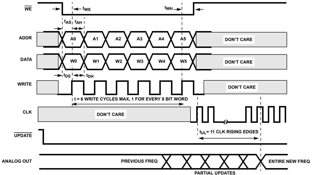
FIGURE 3. PARALLEL-LOAD METHOD 2, \overline{\text{UPDATE}} ACTIVE WHILE LOADING REGISTERS ( \overline{\text{RESET}} = \text{HIGH} )
