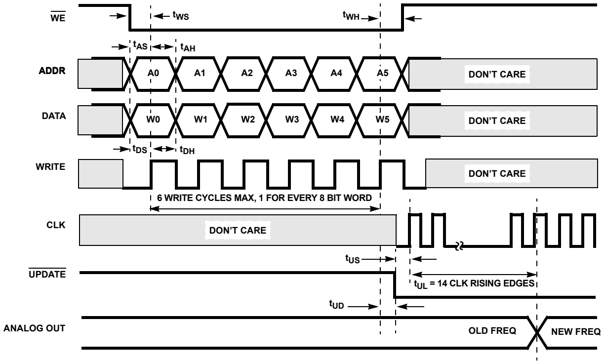
FIGURE 2. PARALLEL-LOAD METHOD 1, \overline{\text{UPDATE}} ACTIVE AFTER LOADING REGISTERS ( \overline{\text{RESET}} = \text{HIGH} )
