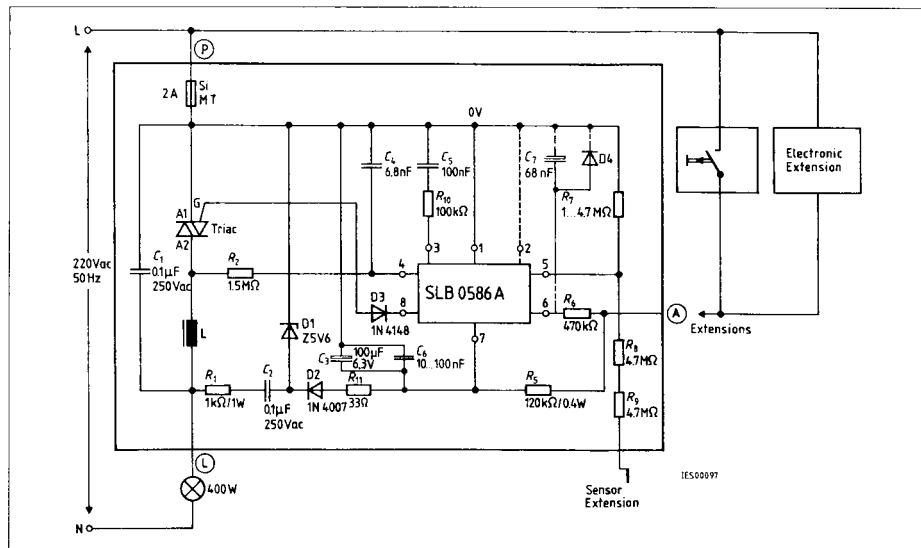
Figure 3 Application Circuit
