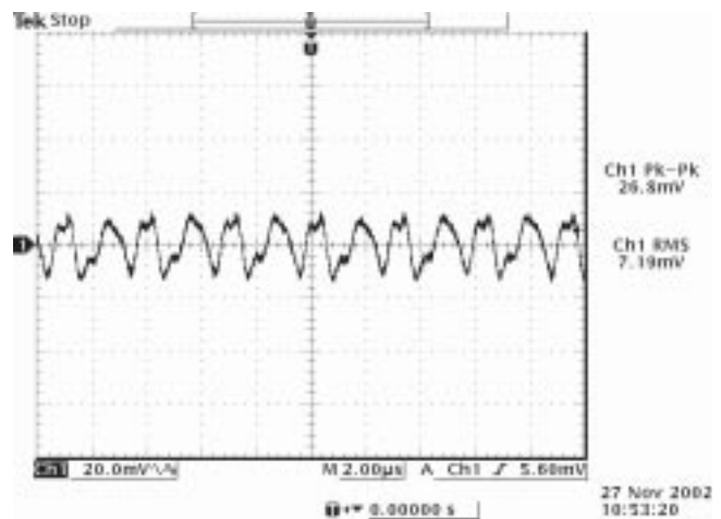
Ripple and noise at full load and 8Vdc input, 1.8Vdc output and Ta=25° C
