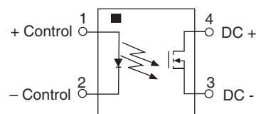
CPC1002N Pinout
