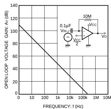
Fig.3 Open loop voltage gain vs. frequency
