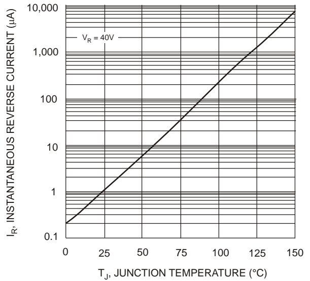
Fig. 4 Typical Reverse Current vs. Junction Temperature
