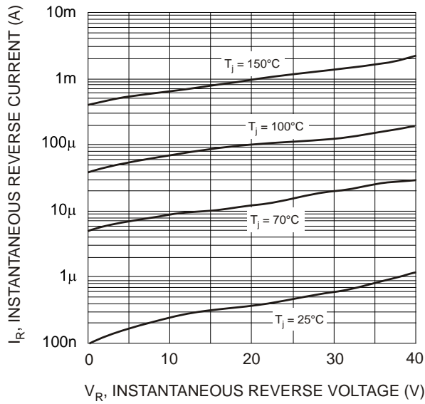
Fig. 3 Typical Reverse Current vs. Reverse Voltage
