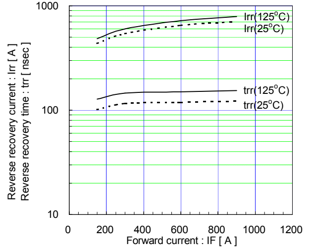
Reverse recovery characteristics (typ.) Vcc=600V, VGE=±15V, RG=0.6Ω
