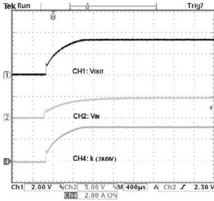
G9966-33 Start-up
