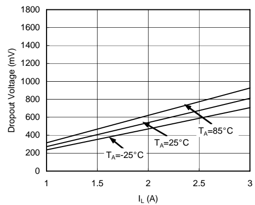
G9966-25 Dropout Voltage vs. I_L
