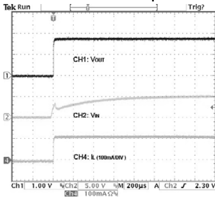
G9966-18-Start-up
