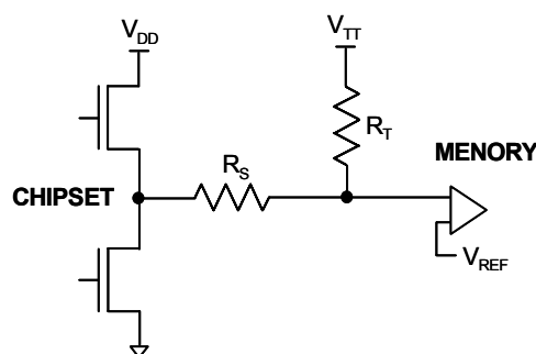
Figure 1. SSTL-Termination Scheme
