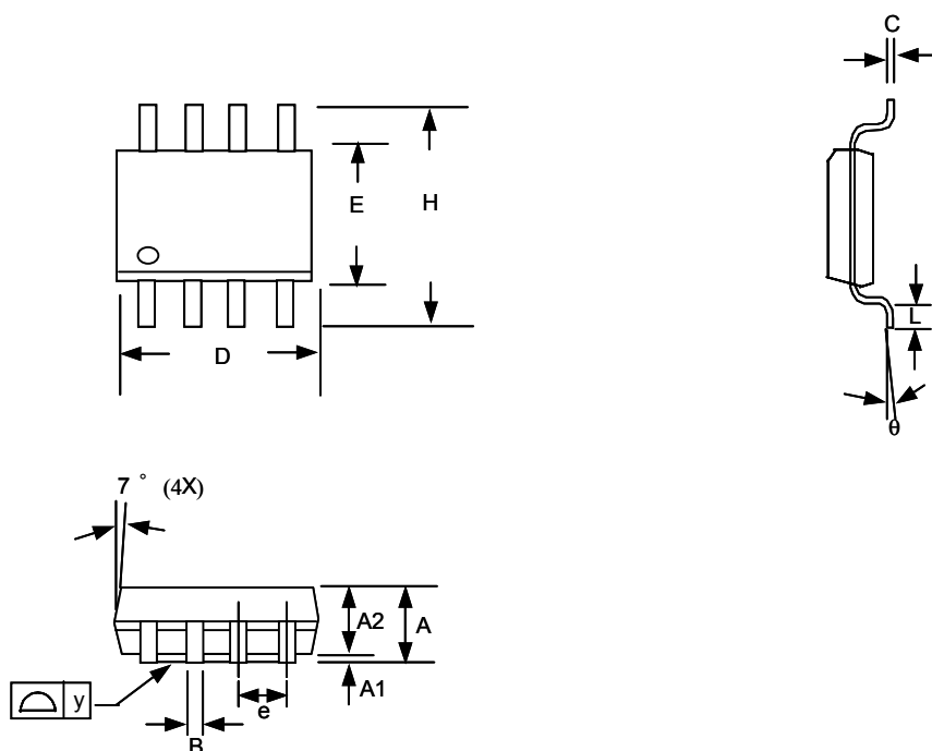
SOP-8L Package
