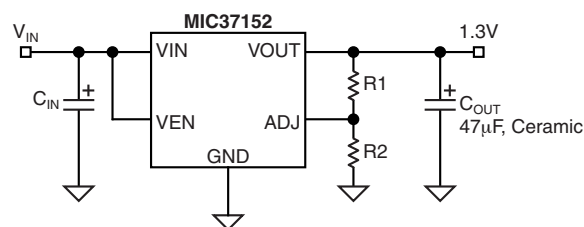
Adjustable Regulator
