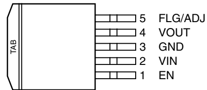
S-PAK-5 (R) MIC37151 MIC37152
