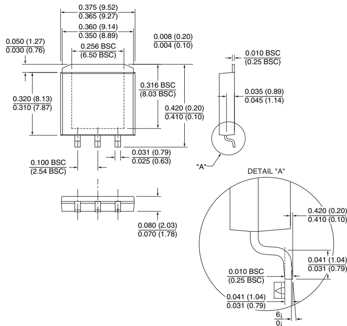
3-Lead S-PAK (R)
