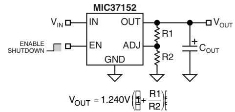
Figure 1. Adjustable Regulator with Resistors
